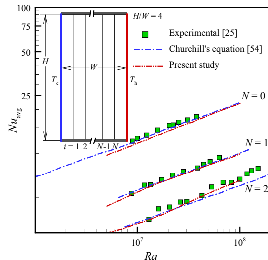
Fig. 7 The comparison of the results obtained by the present study with experimental data [25] and Churchill's relation [54] at AR=4 and Pr = 6
