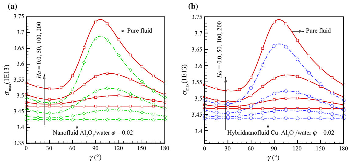
Fig. 17 The effects of Ha and \gamma on the maximum stress imposed on the partition for a the nanofluid with \phi_{\text{Al}_2\text{O}_3} = 2\% and b the hybrid nanofluid with \phi_{\text{hnf}} = 2\% for Ra = 10^8
