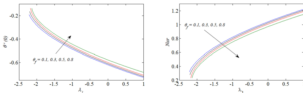
Fig. 8. Variation of \theta'(0) (left) and Nur (right) for \lambda_1 when \phi = 0.05 .
