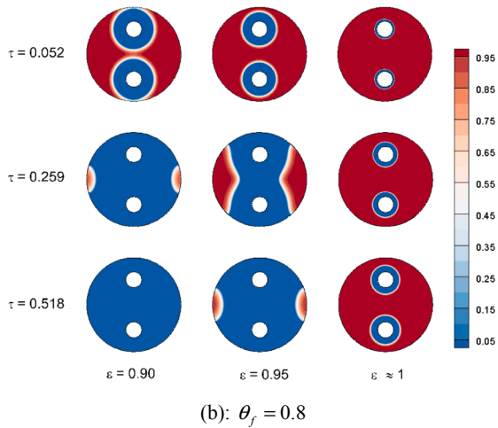
Fig. 16. Discharging state of melting volume fraction rate in different values of porosity and dimensionless melting temperature.
