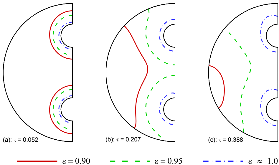
Fig. 13. Displacement of the boundary between solid and liquid interface at MVF = 0.5 during charging mode: \varepsilon = 0.9 , \varepsilon = 0.95 and \varepsilon \approx 1 .
