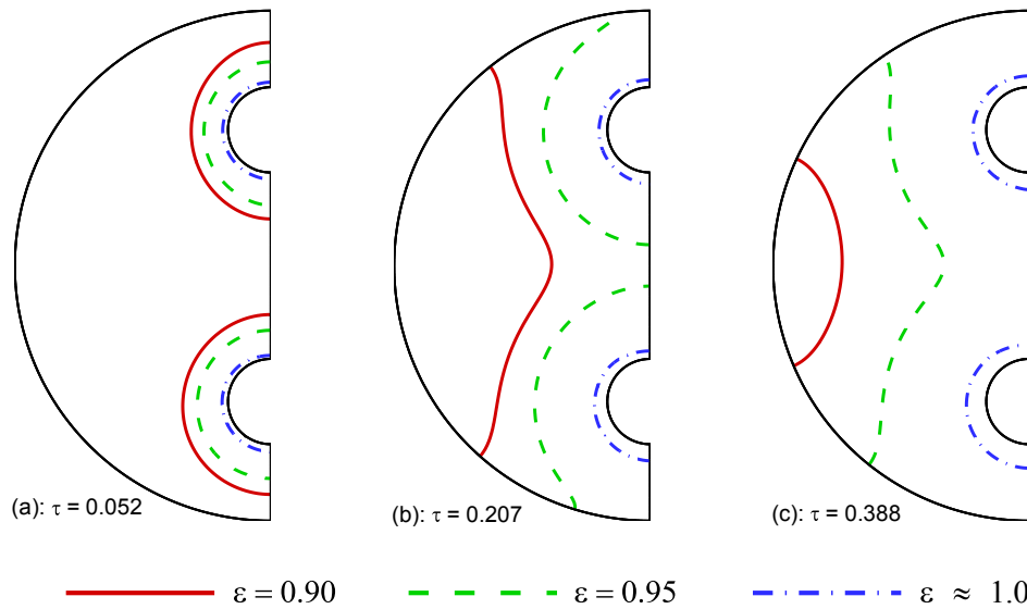
Fig. 12. Displacement of the boundary between solid and liquid interface at MVF = 0.5 during discharging mode: \varepsilon = 0.9 , \varepsilon = 0.95 , and \varepsilon \approx 1 .
