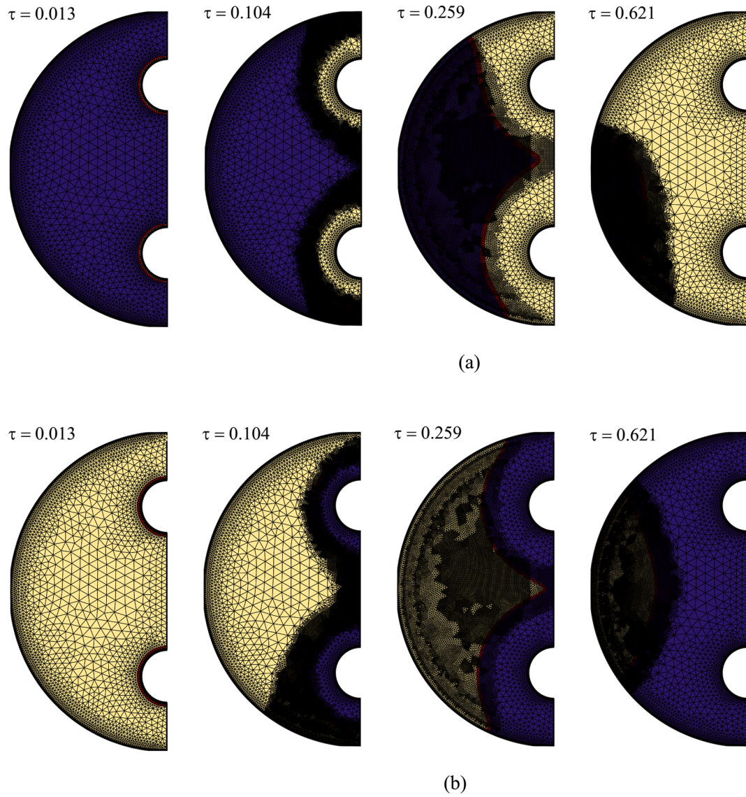
Fig. 4. The mesh adaptation for Case III for (a): melting process and (b): solidification process.
