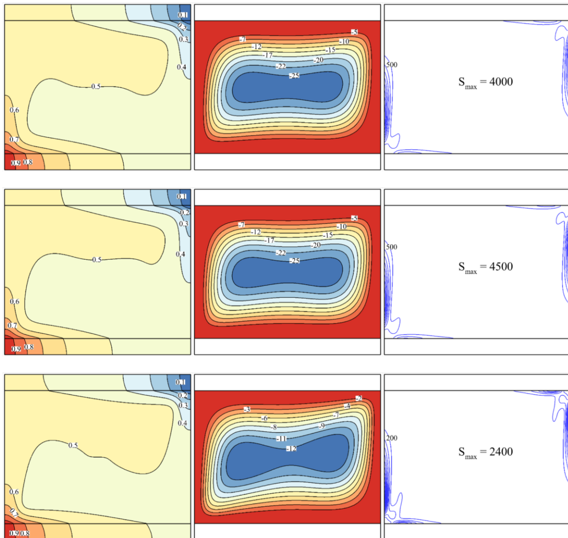
Figure 11. Isotherms, streamlines, local entropy ( S_i ) for selected values of \theta_i (0.1, 0.3, 0.5) at \varphi = 0.05 .
