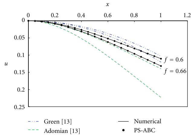
FIGURE 2: Buckling of MWCNT cantilever in the vicinity of graphite sheets for different values of f .
