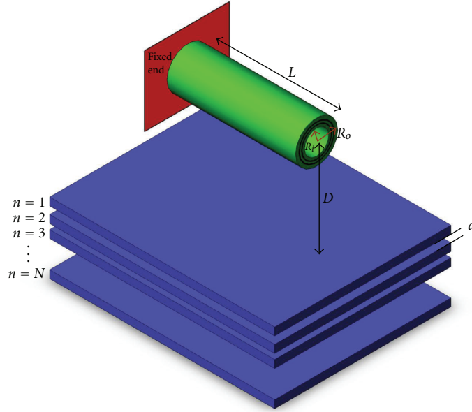
FIGURE 1: Schematic of an MWCNT suspended over graphite sheets.
